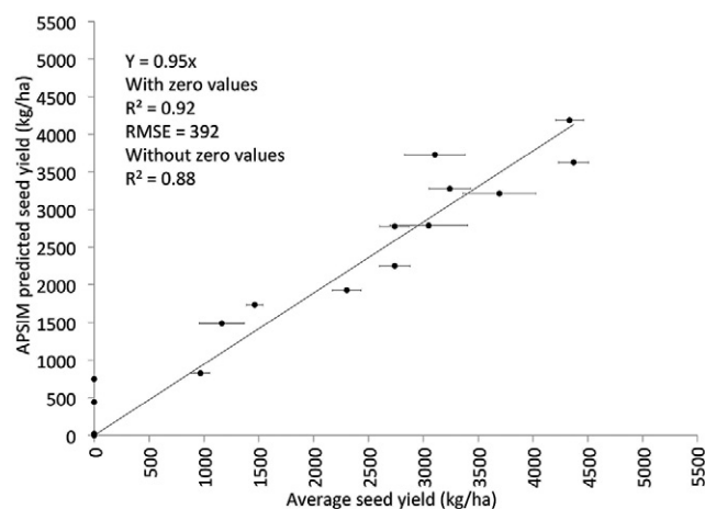
Fig. 4. The relationship between observed field data and APSIM model output of a generic mid-season variety for canola seed yields. The line shows 1:1 relationship. Error bars show standard deviation of field-based seed yield measurements.
